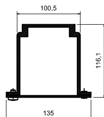
SUPPORTO CASSONETTO HEAD BOX SUPPORT SUPPORT CAISSON
